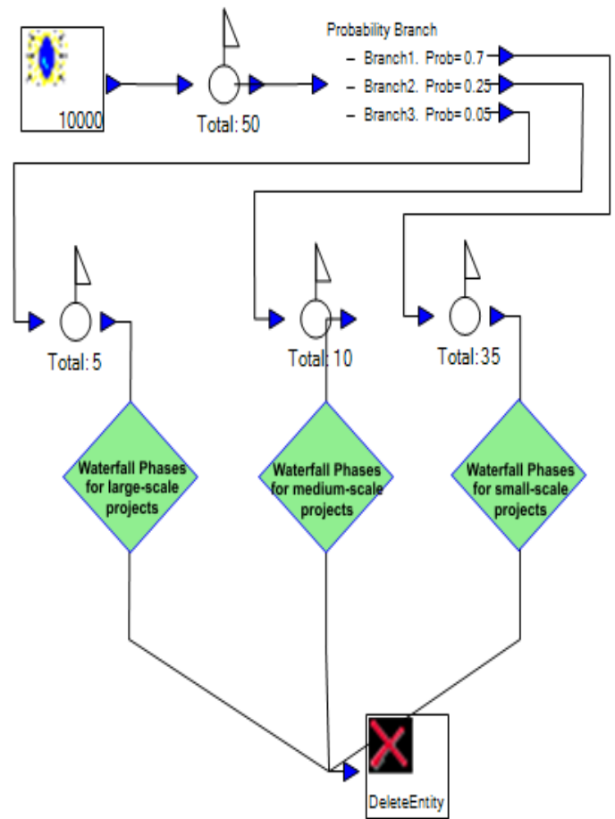
Fig. 3: Simulation model for the Waterfall SDLC
