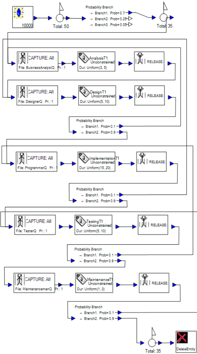
Fig. 4: Simulation model for small-scale type projects
