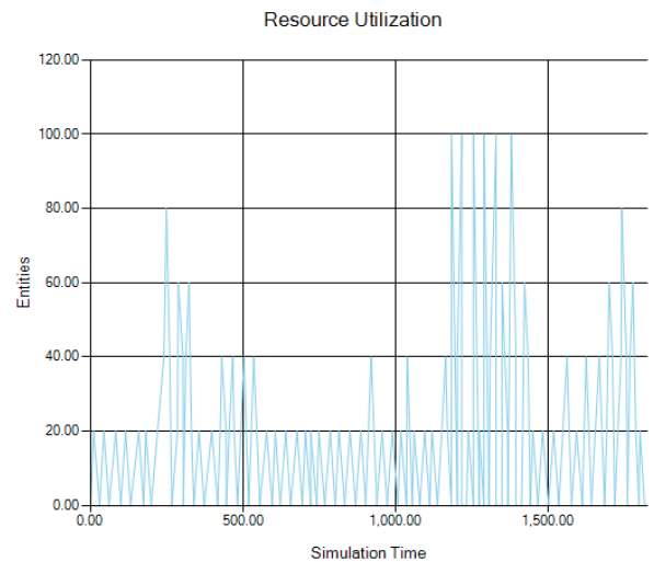
Fig. 5: Utilization of the programmer resource
